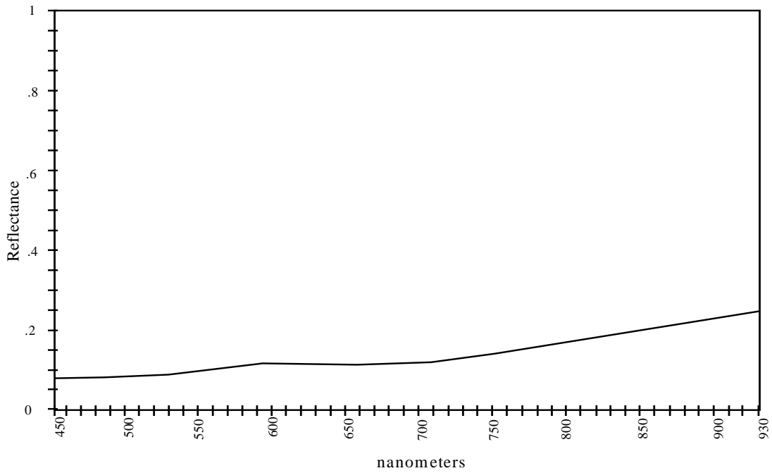
FIGURE C-10. Spectral reflectivity of tree bark.
