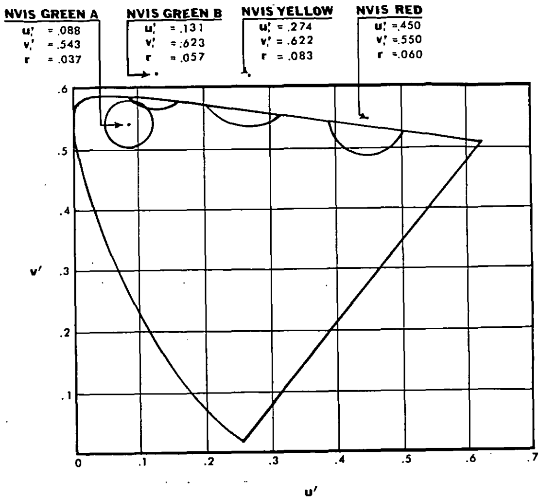
CIE 1976 UCS DIAGRAM
